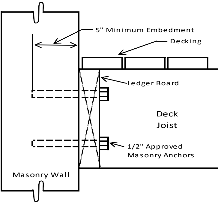
Detail C: Attachment of Ledger Board to Masonry Wall
