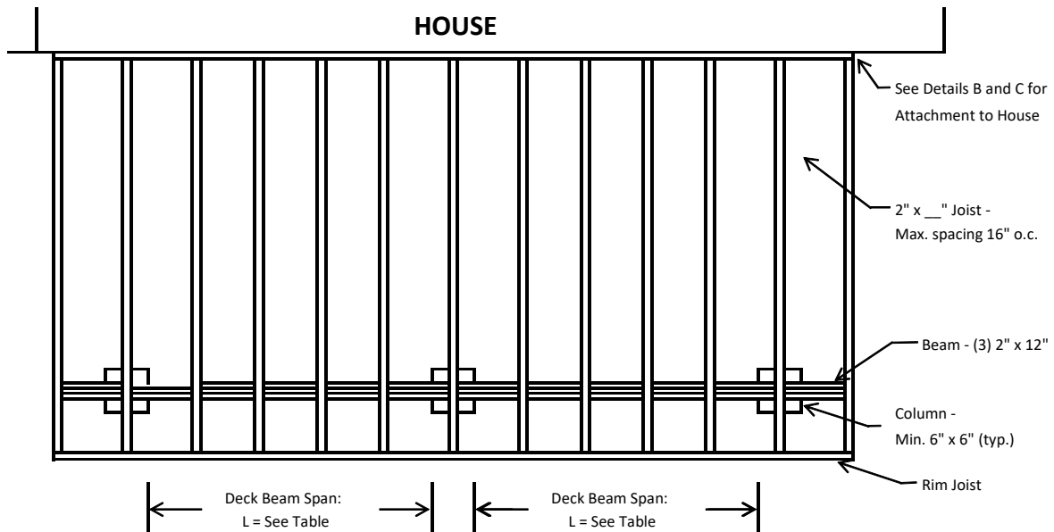
Detail A: Framing Requirements
